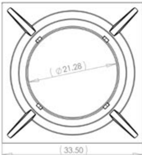
RB-R-26x12 (Riser)
